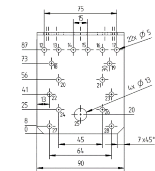
Figure A.33 Angle Bracket 8626 10PL 1
